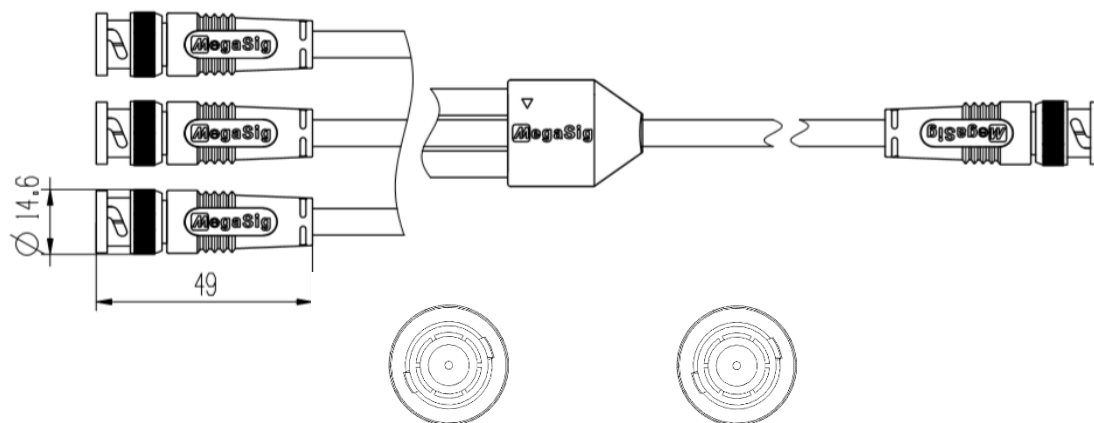
BNC Plug
